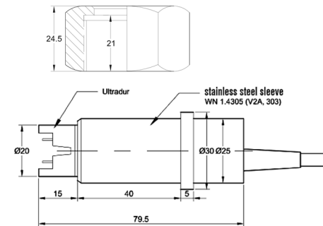
Type 3205.30: Techn. Data as 3202.30 max. pressure 10 bar, installation with union nut G 1" A, SW 37 mm, DIN 259, ISO 228 mass approx. 200 g without nut
