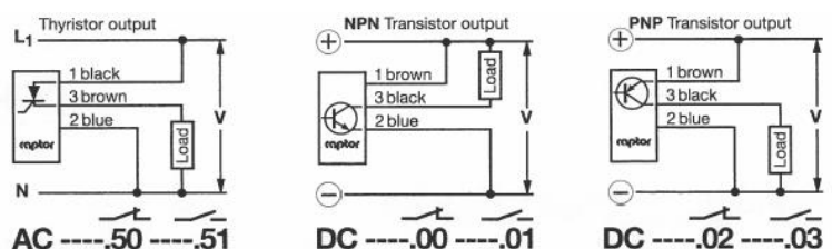
connection diagram
